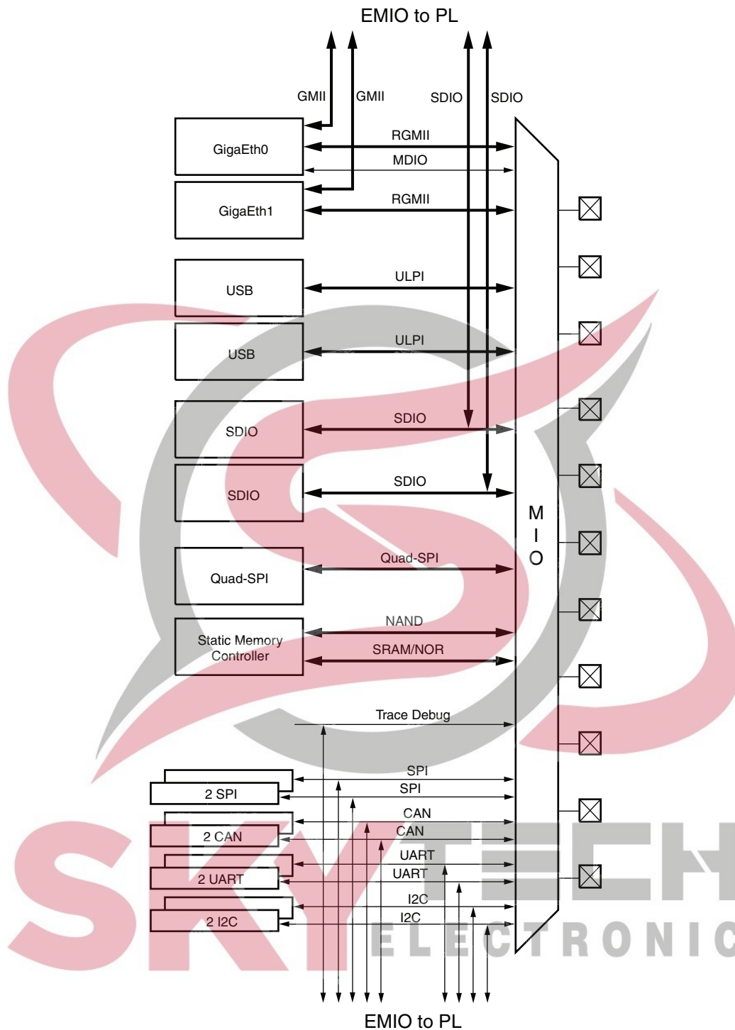
Figure 2: MIO Module Block Diagram
